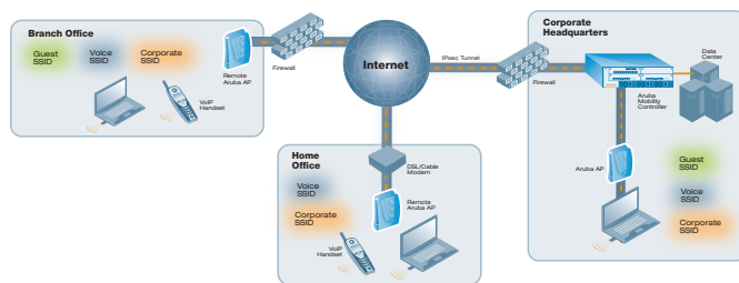
Aruba Remote APs are ideally suited for providing secure mobile connectivity to branch and home offices. All security policies are centrally defined and enforced on Aruba's mobility controller.
